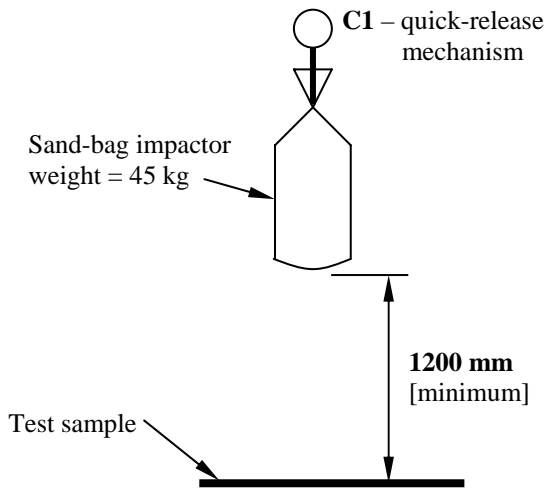
FIGURE A2/2 – Arrangement for drop-test [2.3.3]
