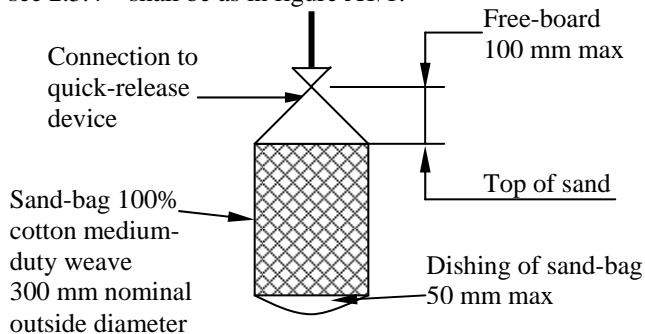
Figure A1/1 – Sand-bag for drop-test
