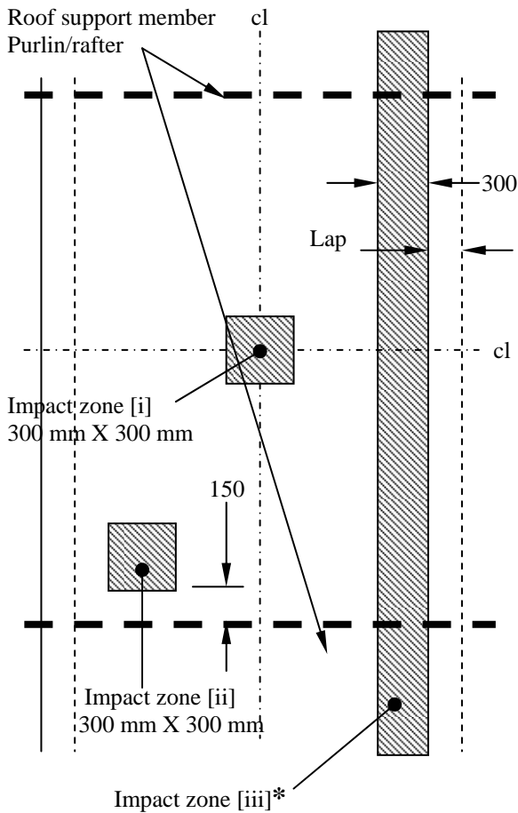
FIGURE A2/2 – Arrangement for drop-test [2.3.3]
